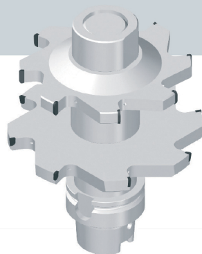
PCD double cutter Piston side cutting
